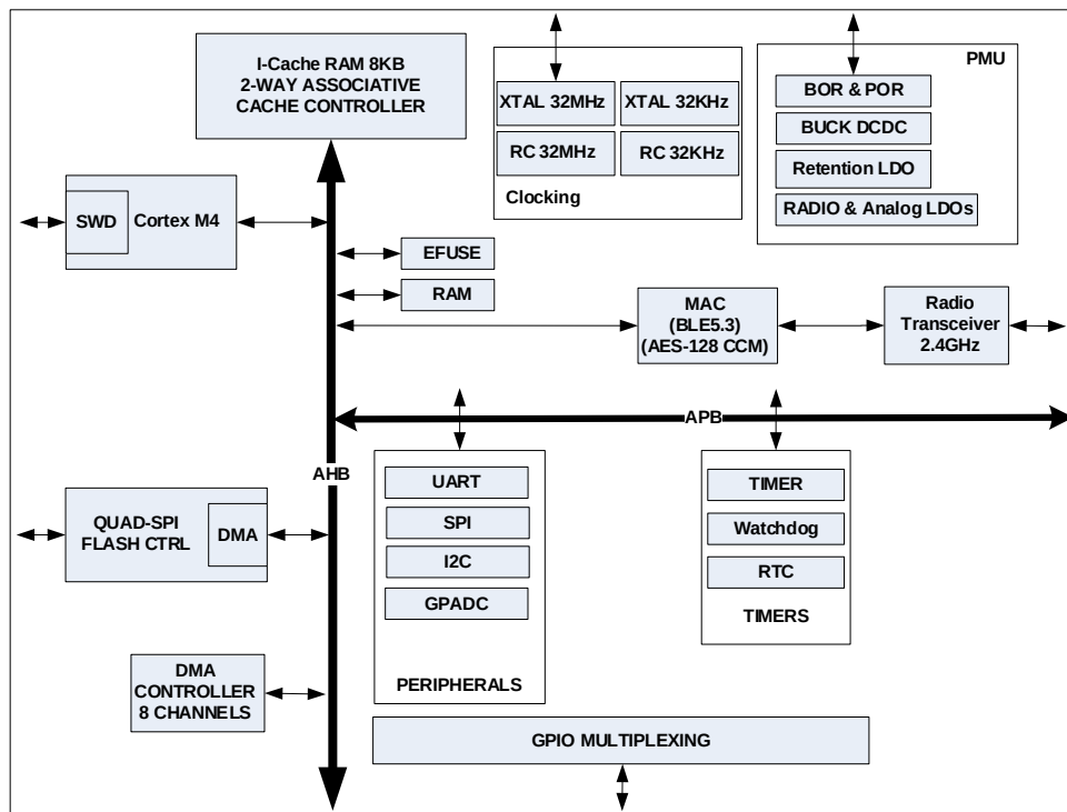
Figure 3.1 Micro-controller Subsystem
